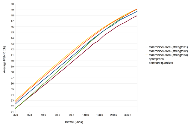
Koishi 480p
