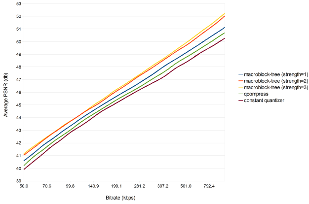
deadline CIF
