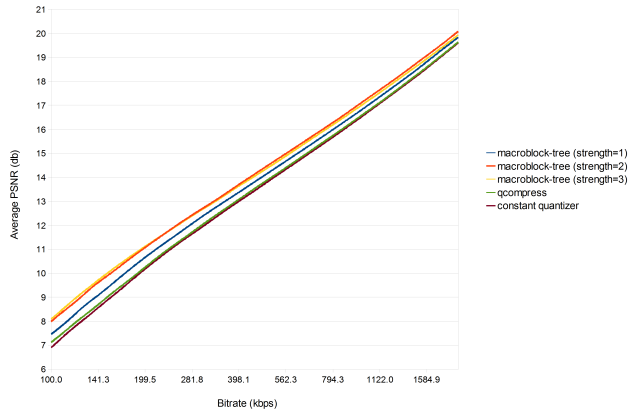
mobile CIF
