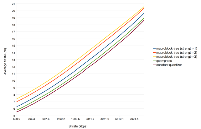
Koishi 480p
