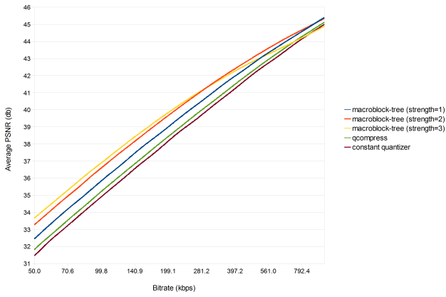
mobile CIF
