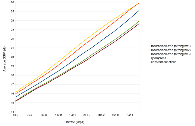
deadline CIF
